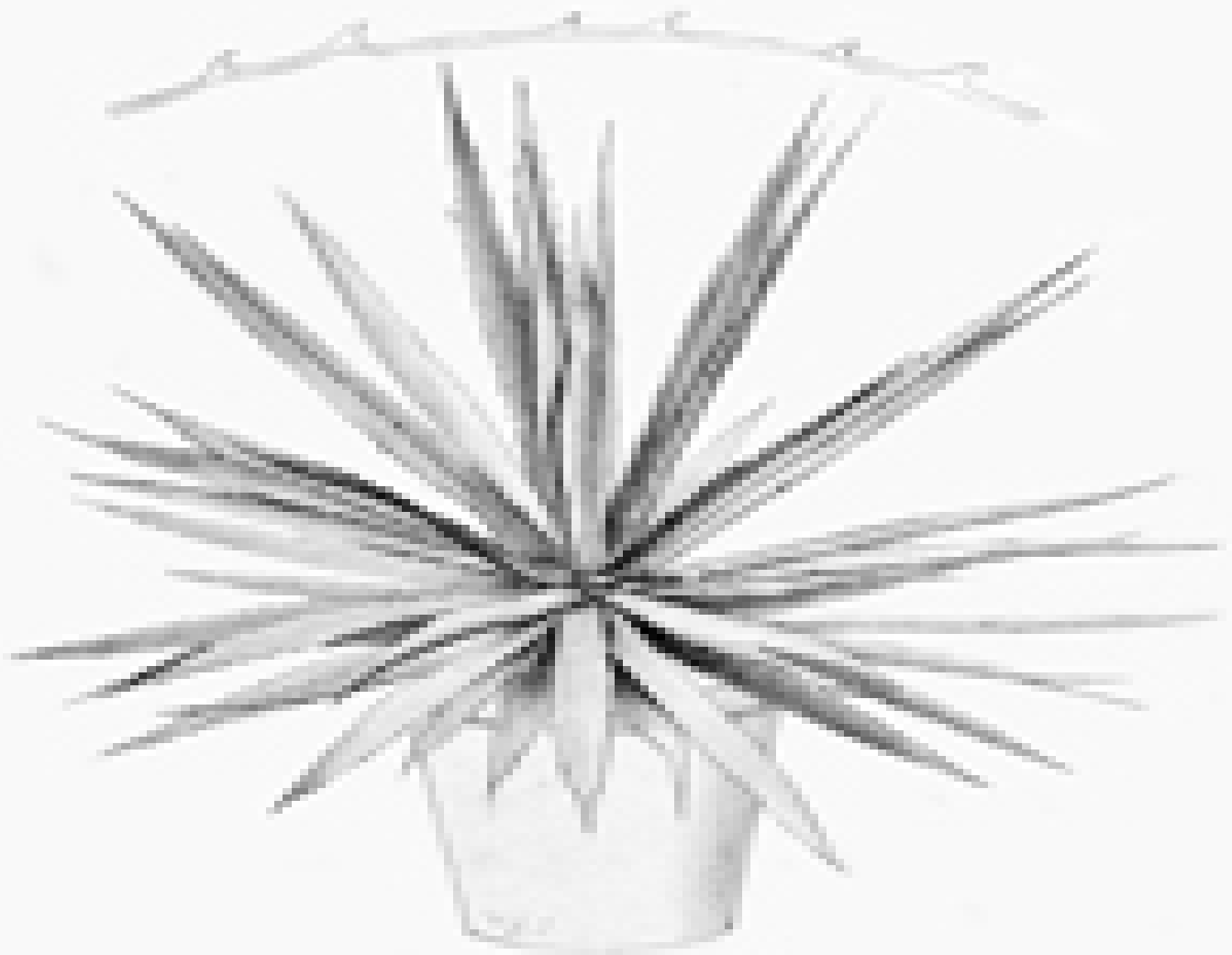
Fig. 58. — Agave unimulata
